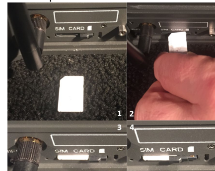
Installing SIM card and engaging the lock
